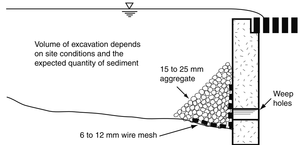
(b) Details of the weep hole and aggregate placement
