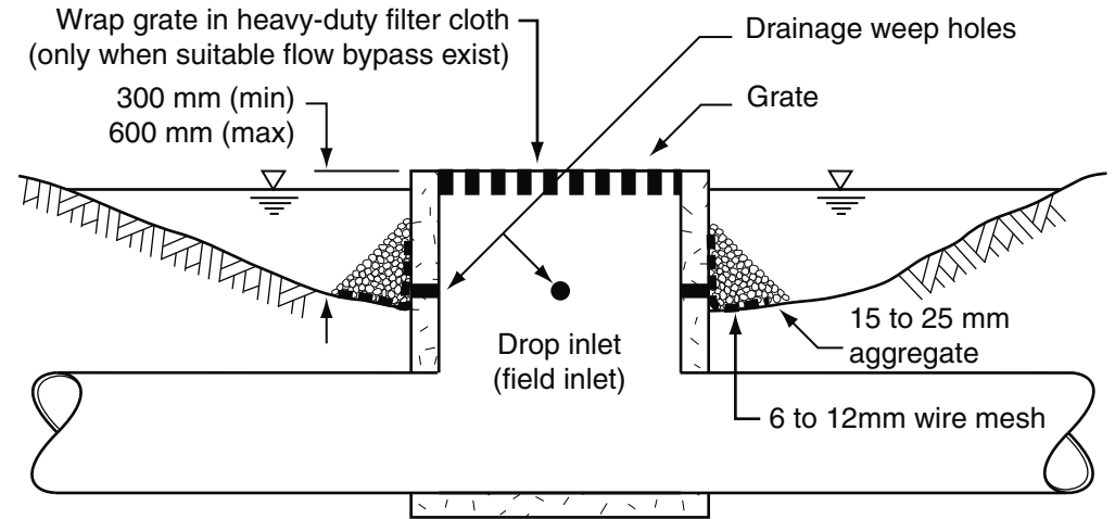
(a) Typical layout of excavated drop inlet protection
