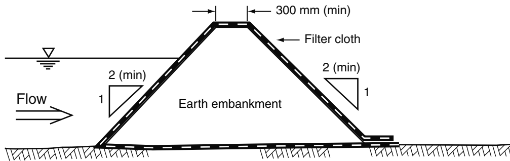
(c) Typical details of a temporary earth abutment
