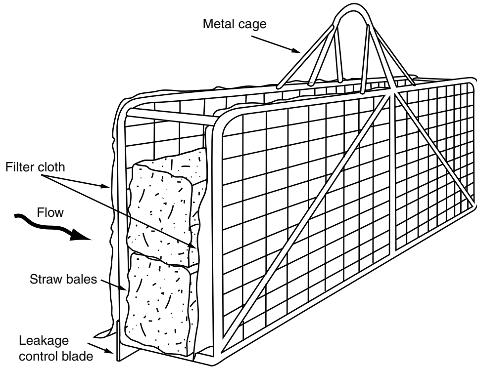
(a) Sediment filter cage
