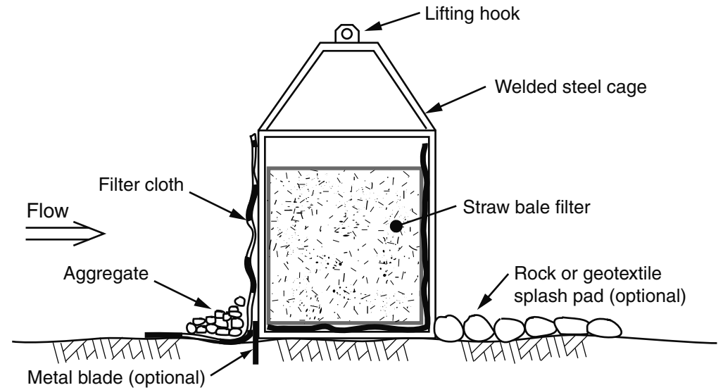
(b) Typical installation details for a sediment filter cage
